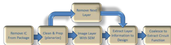
Fig. 1. Traditional deprocessing workflow based upon SEM imaging. Graphic adapted from David Weaver, et al., “Fast Mask Data Recovery to Provide Missing/Incomplete Technical Data Packages (TDP) for Obsolete ICs and Validating Trust Within ICs”, GoMACTech 2011.
