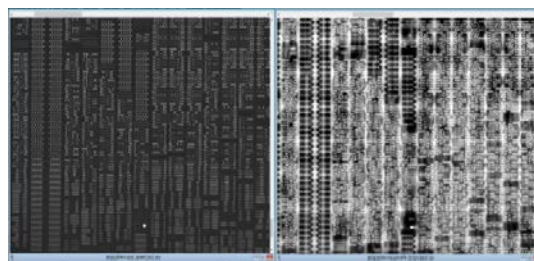
Fig. 7. Gate structures highlight at 5kV BSE, shown on the left and looking into M1 in the 30kV BSE image at right. Both images are a montage of 49 images @ 4096x4096 pixels each.
