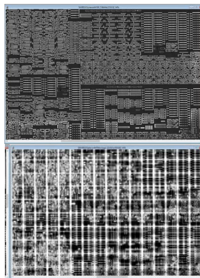
Fig. 8. Contact layer is prominent in the 5kV BSE montage image at top while the 30kV BSE image montage is looking into M2/M3 (bottom). Both images are a montage of 49 images @ 4096x4096 pixels each.
